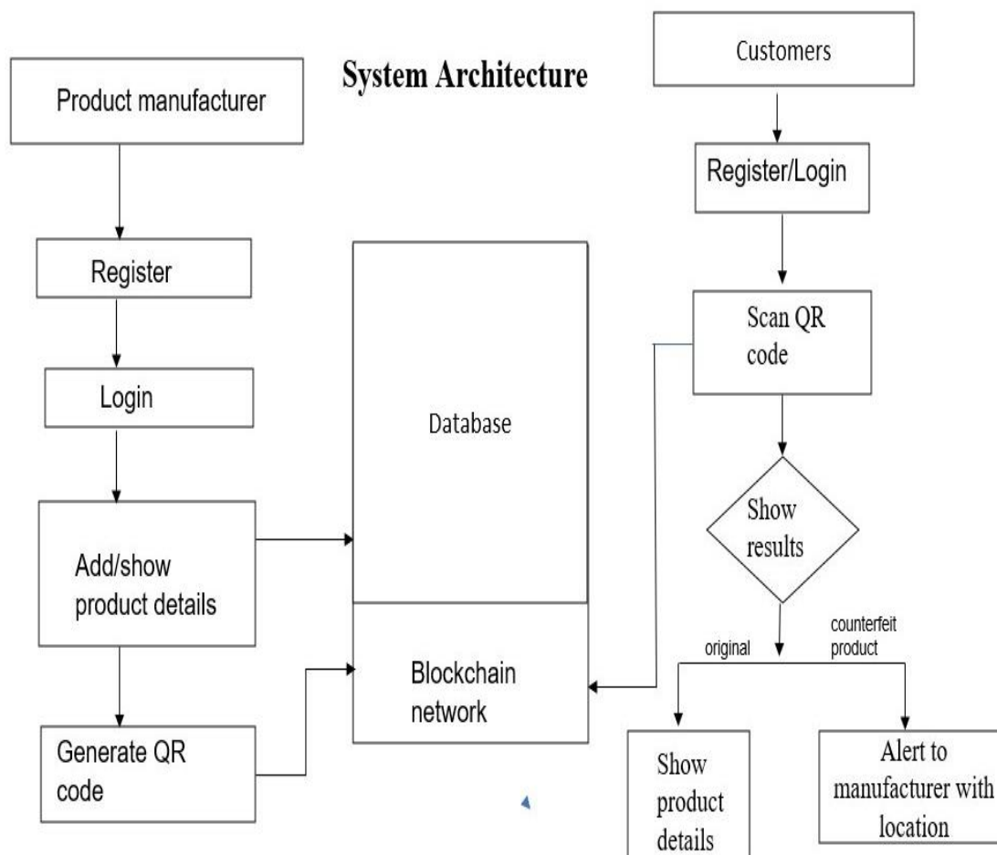
Fig 2: System Architecture
