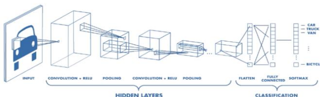
Figure 2: CNN Model
