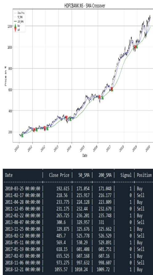
Fig.3. Algorithmic Trading Strategy
